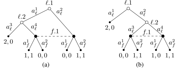
Figure 1: Examples SEFGs.
