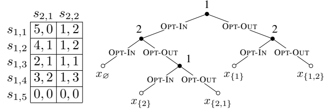
Figure 1: Left: Example of two-player normal-form SG with L = \{1, 2\} . Right: Sequential game representing its agreement stage.
