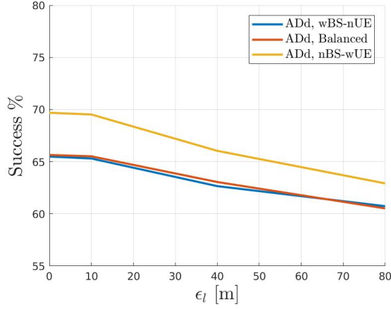
Fig. 3. iBWS success rate. No Obstacles.
