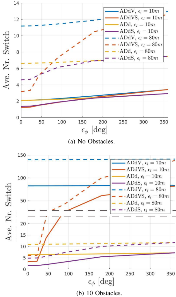
Fig. 6. Algorithm performance comparison. ADdVS+ at BS side. nBS-wUE iBWA strategy.
