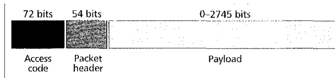
■ Figure 3. The format of packets applied in Bluetooth.
