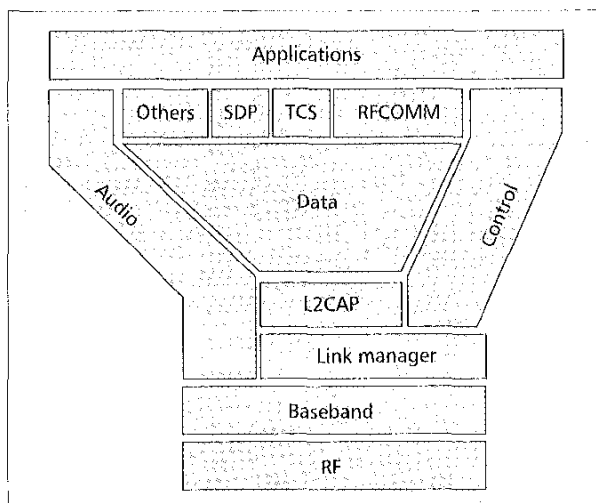
■ Figure 12. The Bluetooth protocol stack.
