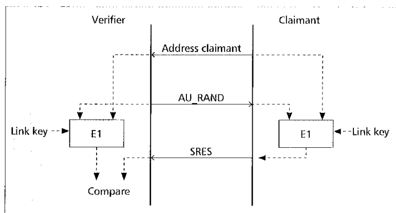
■ Figure 11. The Bluetooth authentication procedure.
