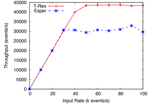
Figure 5: Filtering: Comparison Between T-Rex and Esper
