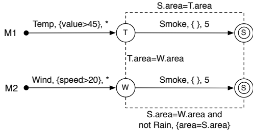
Figure 2: Event detection automata for Rule R7
