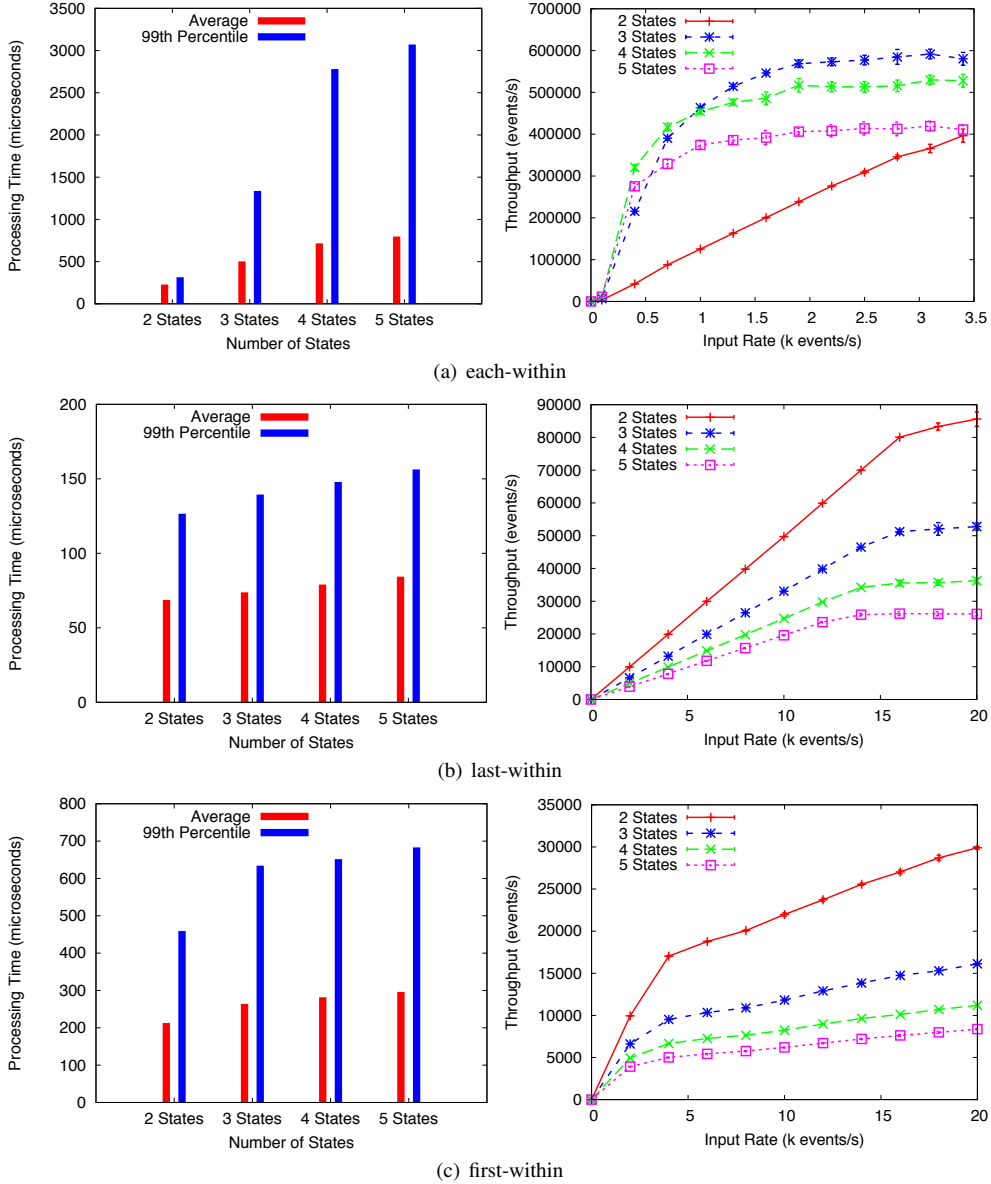
Figure 8: Number of States in Sequences
