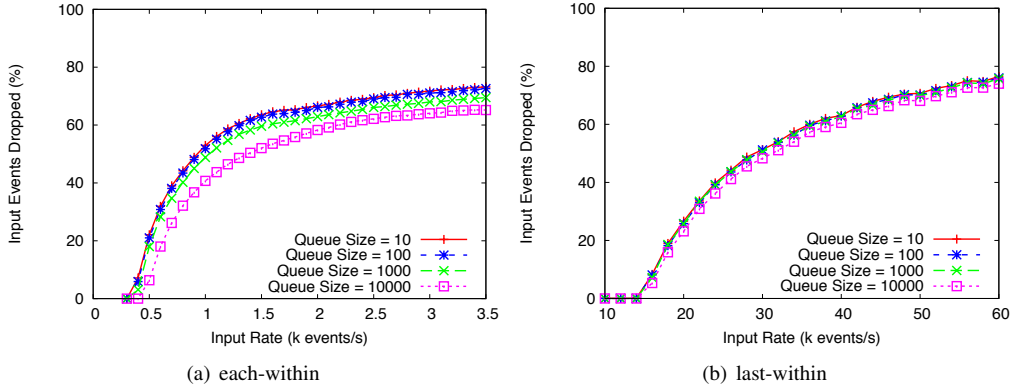
Figure 16: Size of the Input Queue
