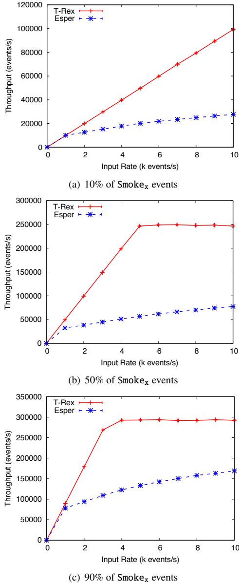
Figure 7: Comparison Between T-Rex and Esper Using Rule R5
