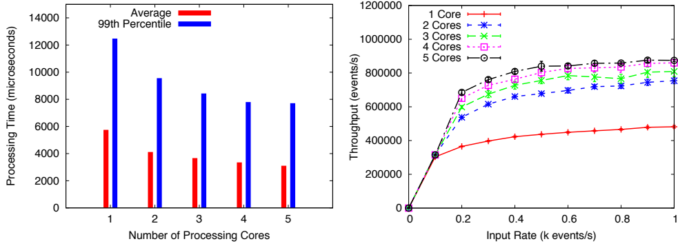
Figure 13: Scalability
