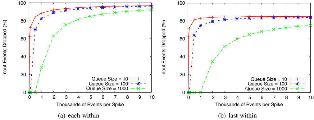
Figure 17: Tolerance to Spikes
