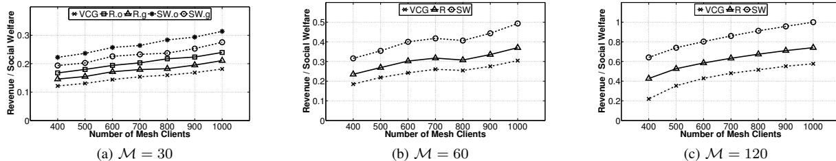
Fig. 2: Revenue and Social Welfare measured as a function of the number of mesh clients in scenarios with 30, 60, and 120 mesh devices.
