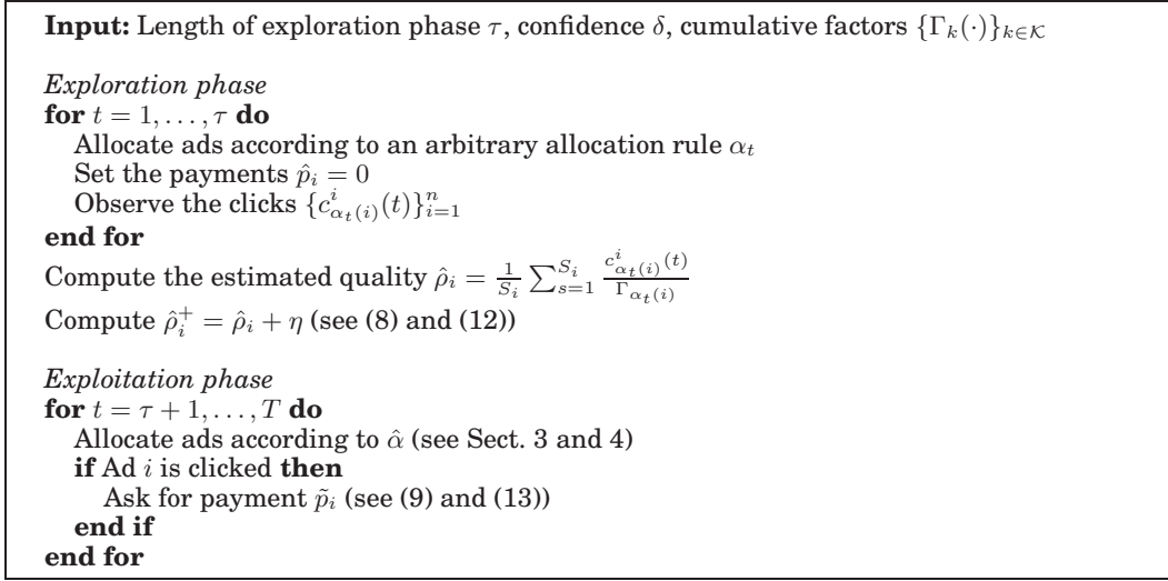
Fig. 1. Pseudo-code for the A-VCG mechanism.
